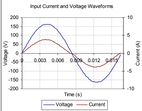
Input AC Current Waveform (ITHD = 8.97%, 50% Load)
