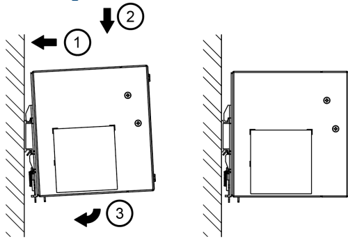
Fig. 3.1 Mounting
