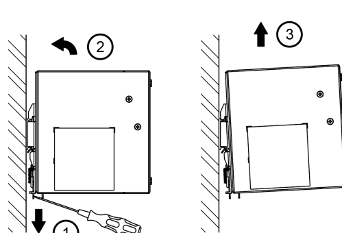
Fig. 3.2 Dismounting
